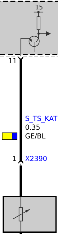
B2390 Exhaust temperature sensor be- fore catalytic converter
