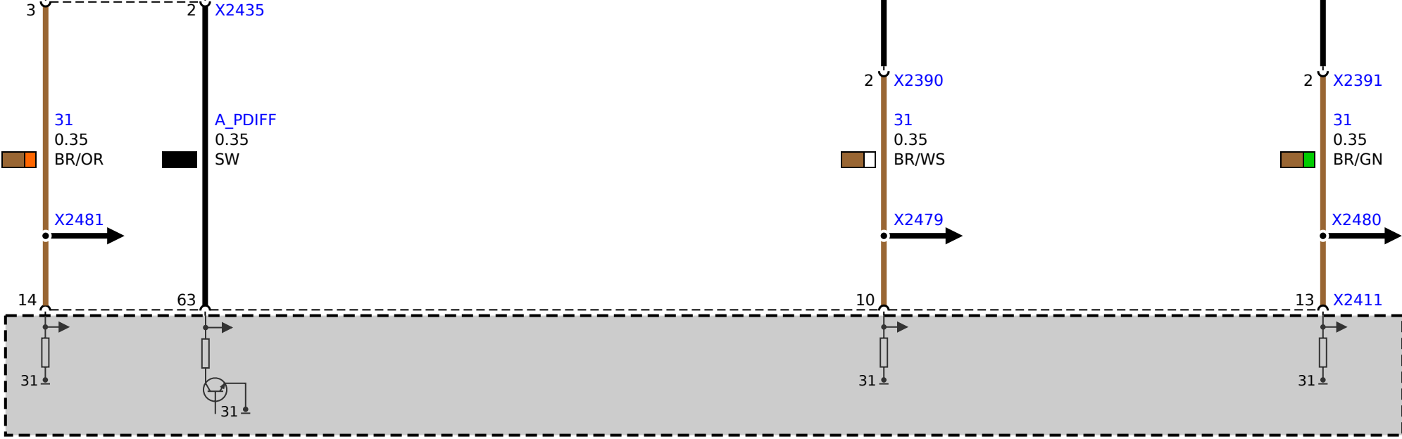
A460 Digital diesel electronics
