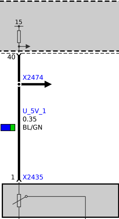
B300 Exhaust gas pressure sensor before diesel particulate filter
