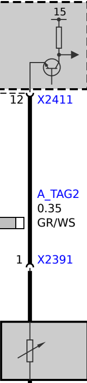
B315 Exhaust temperature sensor upstream of diesel particulate filter
