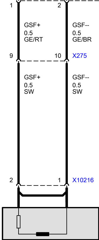
G12 Belt tensioner, driver
