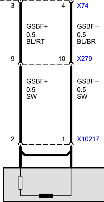
G13 Belt tensioner, passenger
