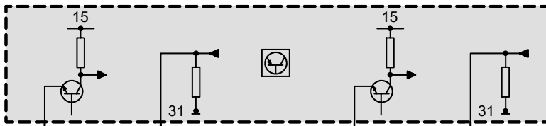
A12 Multiple restraint system control unit
