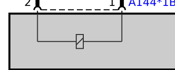
A144 Holding magnet, parking lock
