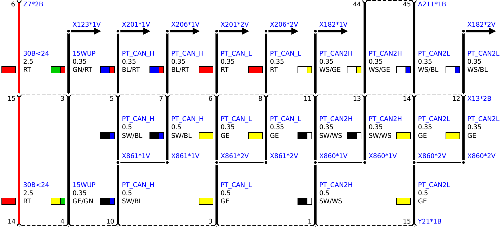
Y18 Twin-clutch gearbox
