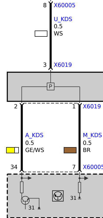
B6125a Low pressure fuel sensor
