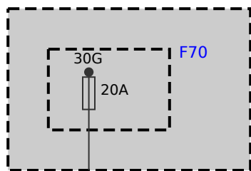
A4010 Junction box
