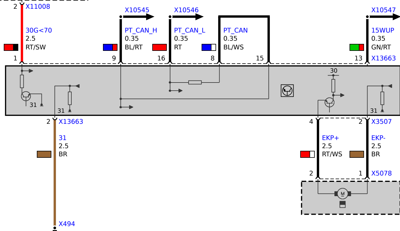
A13663 Fuel pump control (EKPS)
